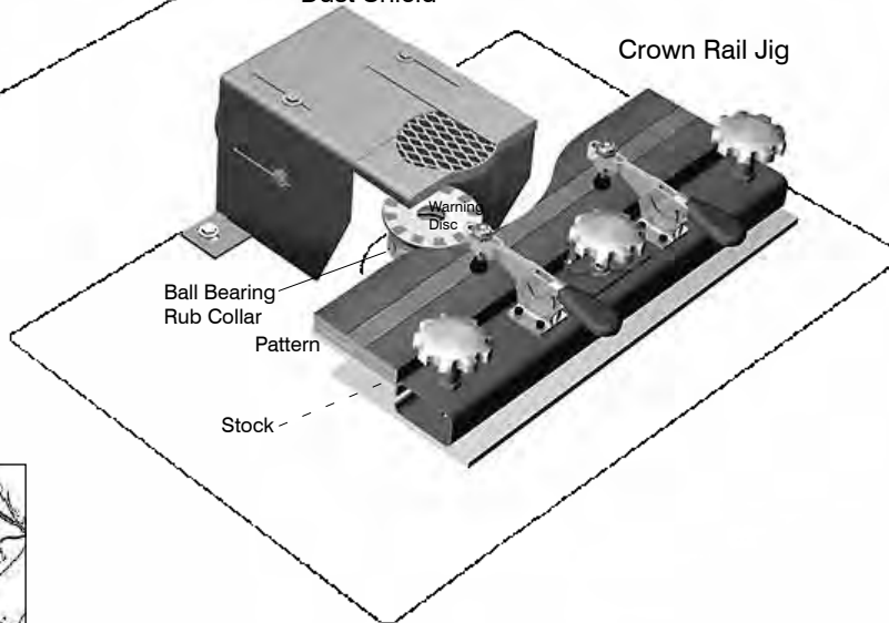
Dust Shield
