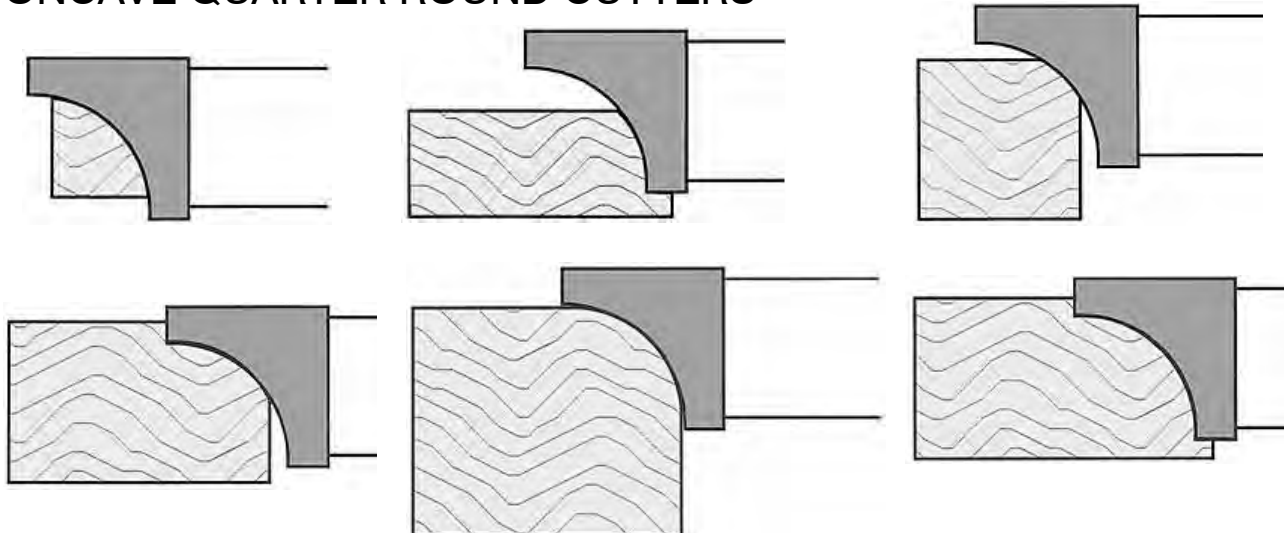
CONCAVE QUARTER ROUND CUTTER EXAMPLES
