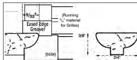
Brazed Tip Stile & Rail Set For Glass Doors - Stile Half
