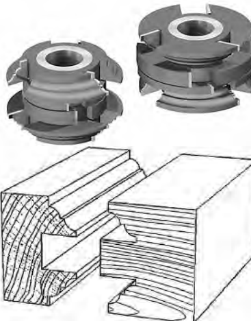
Example Cut
