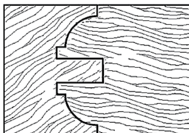
1 3 / 8 " Interior Profile, using one spacer & the 1/4" groover.
