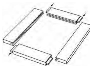
Shaker door tenon exploded view.
