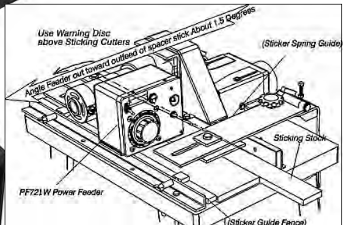
Warning Disc
