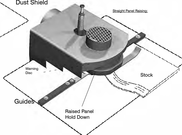
Dust Shield
