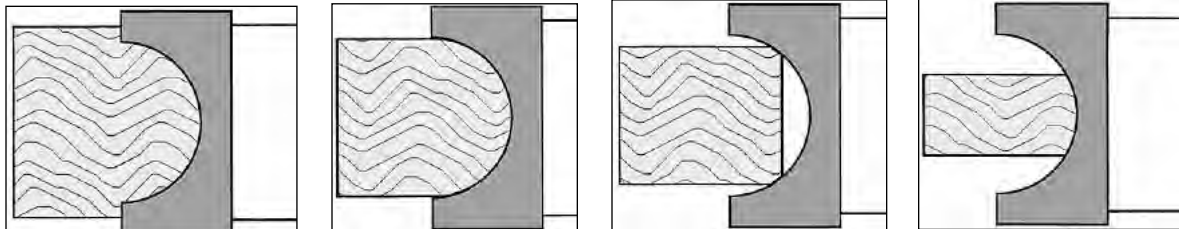
CONCAVE HALF ROUND CUTTER EXAMPLES
