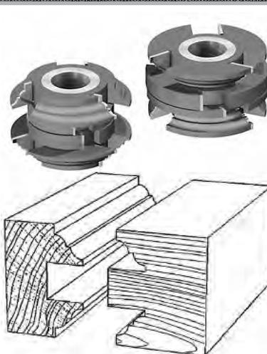
Example Cut
