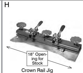
Crown Rail Jig
