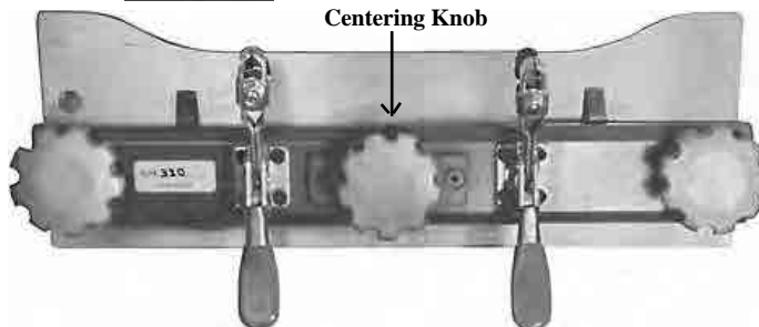
Centering Knob
