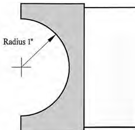
1" Radius Concave Half Round Edge Cutters
