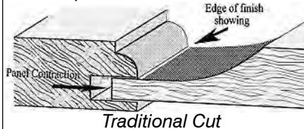
Traditional Cut
