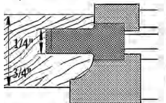
Traditional Cut
