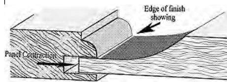
Traditional Cut
