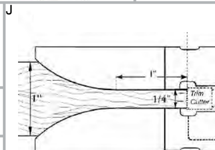
305-SB Double Raised Panel Cutters
