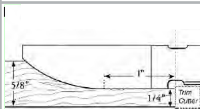
305-SA Single Raised Panel Cutter
