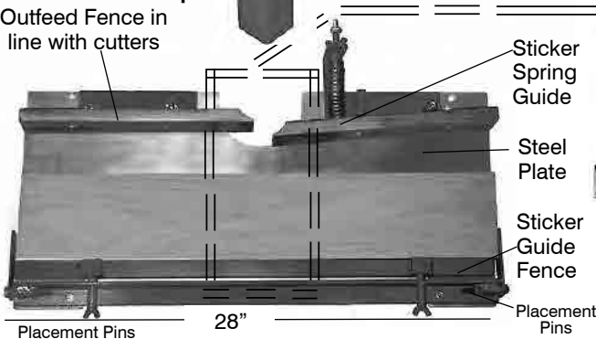
Flat Mount General Hold Down - Included w/Sticker Plate
