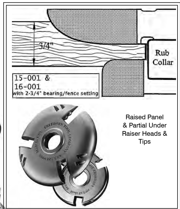
Shapermaster
