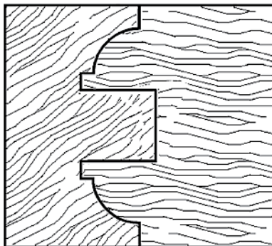
1\frac{3}{4} " Exterior Profile using 2 spacers & the \frac{9}{32} " & \frac{1}{4} " groovers.
