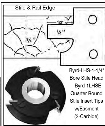
Easement Cut
