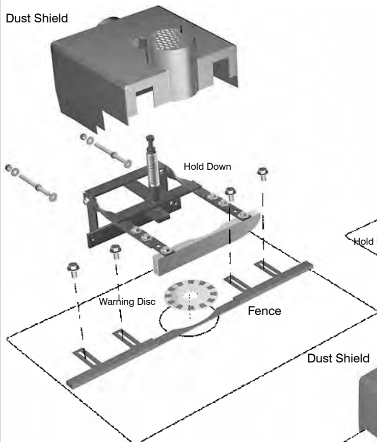
Dust Shield
