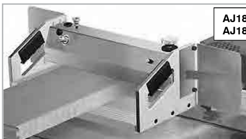
AJ1801LW 18" Air Tenon Jig "left", clockwise cutter rotation.
