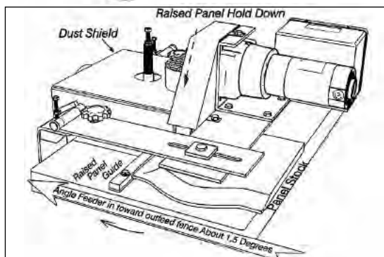
Straight Panel Raising Shaper MANUFACTURED IN U.S.A.
