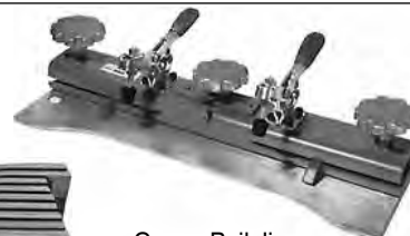
Crown Rail Jig
