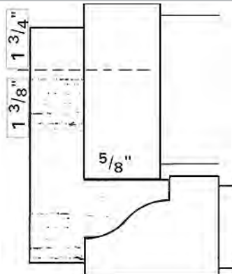
Spindle Spacers
