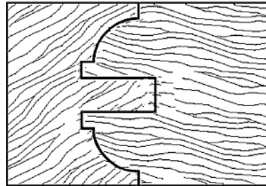
1\frac{3}{8} " Interior Profile, using one less spacer & the \frac{1}{4} " groover.
