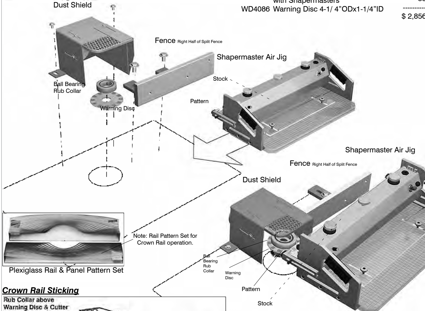
Dust Shield
