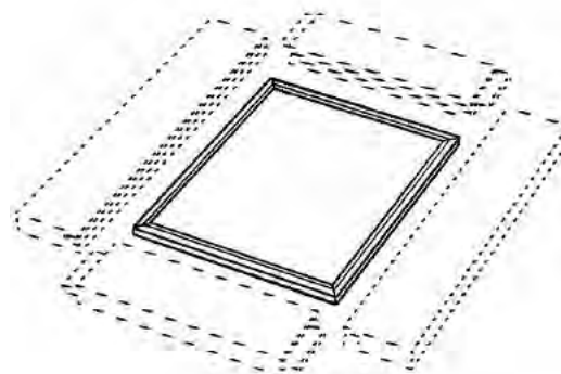
Shaker door exploded view backside with 'partial raised' panel.
