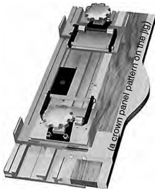
JM310 Crown Panel Jig
